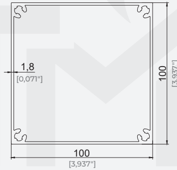
100x100 Dikme Profil 100x100 Pillar Profile
