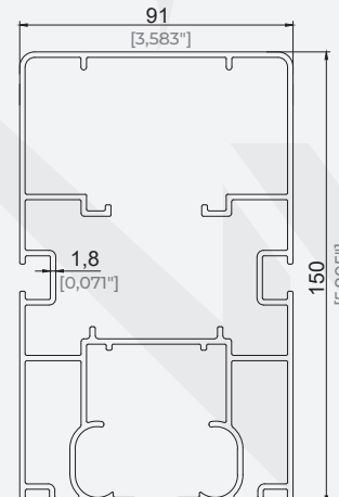
91x150 Eko Ray Profili 91x150 Eco Rail Profile
